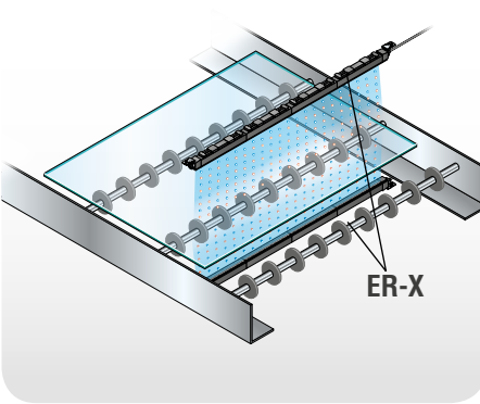
Eliminating static electricity when transporting glass circuit boards
