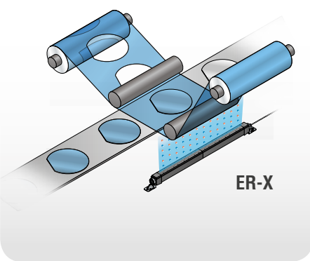
Eliminating static electricity when separating protective tape
