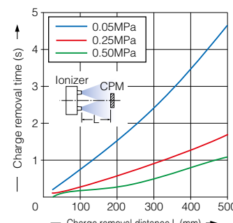
Correlation between charge removal distance and charge removal time
