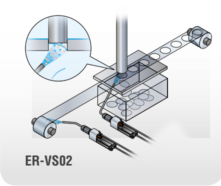
Keeping punched-out material from sticking to punches
