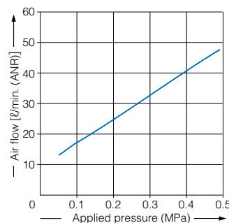
Air flow
