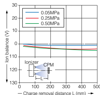
Correlation between charge removal distance and ion balance
