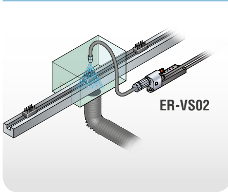
Removing dust from connectors and switches
