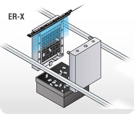
Preventing adhesion of molded parts to molds
