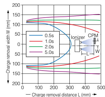
Charge removal field (0.50MPa)
