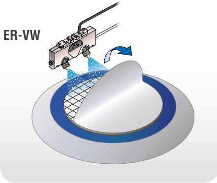
Removing static electricity during background sheet separation
