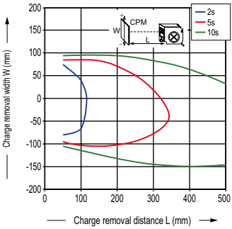
Charge removal field (vertical direction) (fan speed MAX, filter is mounted)
