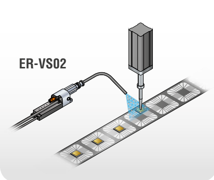
Preventing electrostatic damage during bonding
